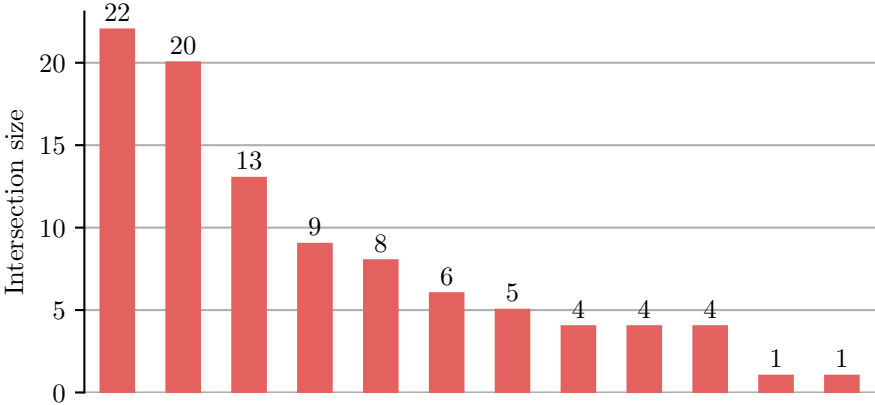
Shrinkage Intersections (pass@256 Base=1, RL=0), Model: EuroLLM-9B-Instruct
